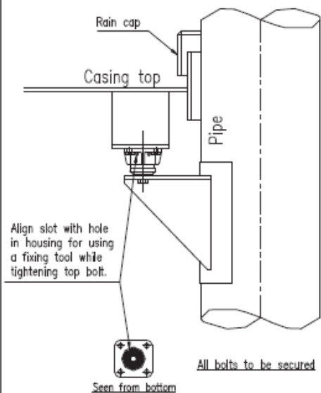
Fix point support at top penetration
